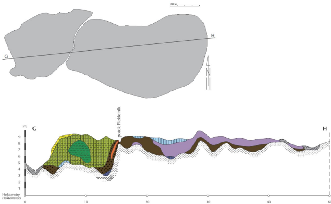
Figure 1.4.3: Peat stratigraphy of Baligówka bog, by Lipka & Zajac
