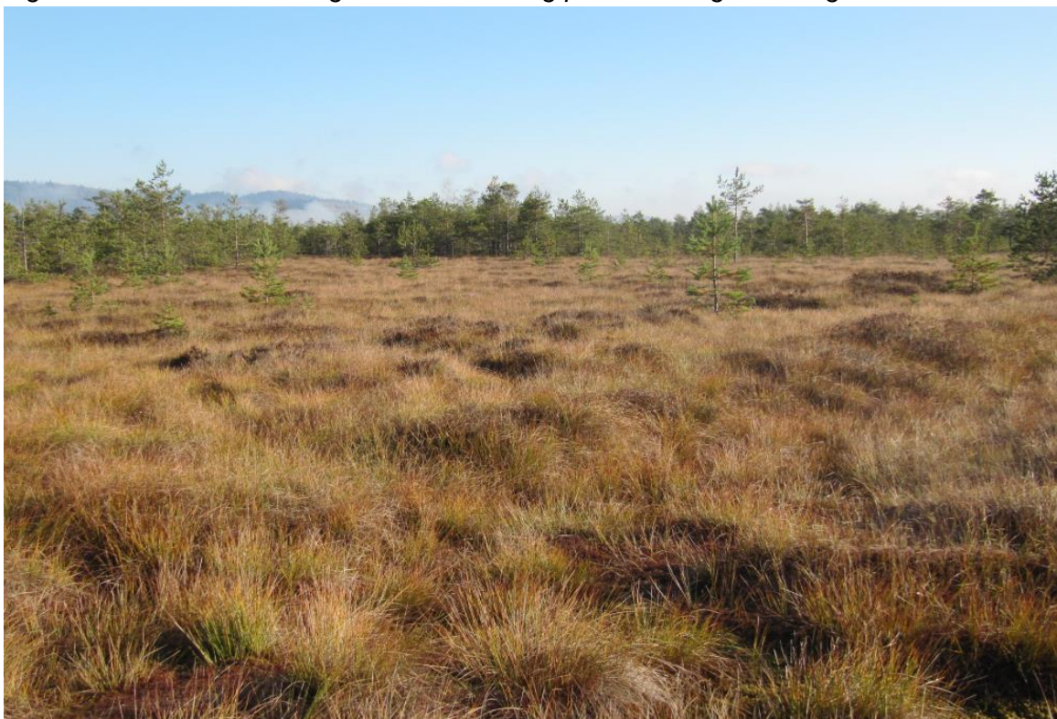
Figure 3.4.3: Open part of the Baligówka bog ( Eriophoro vaginati-Sphagnetum )
